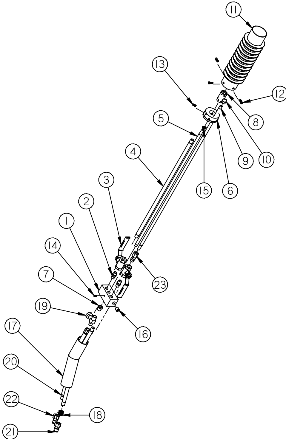
Figure 6.1 Hot Air Lance
