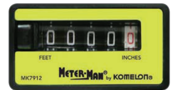
Kickstand Molded into Counter Housing
